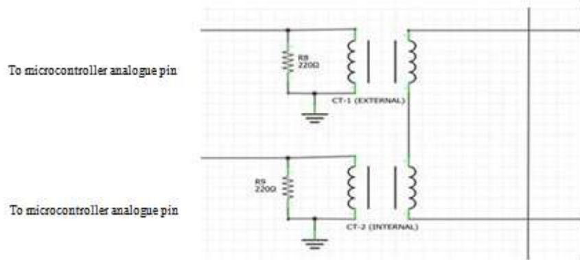
Figure 3. Meter by-passing circuit
