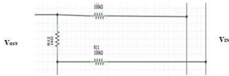
Figure 2. Voltage divider circuit
